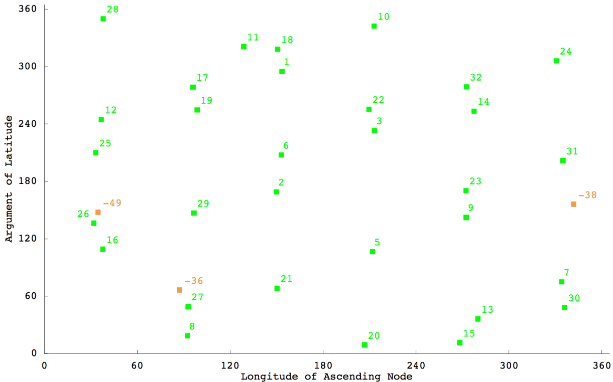
GPS Satellite Constellation (GPSWeek 2009(985); GPS Seconds 518400)
