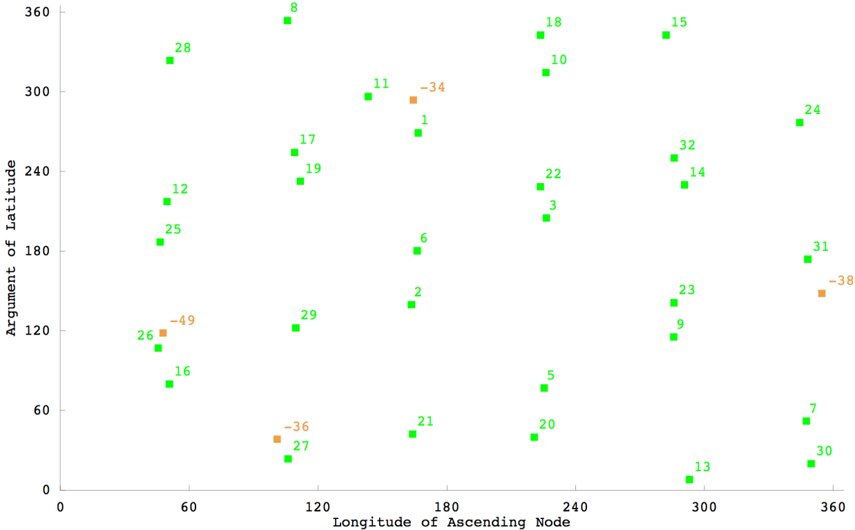
GPS Satellite Constellation (GPS Week 1957(933); GPS Seconds 518400)
