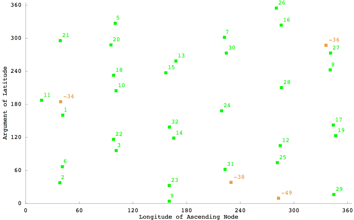
GPS Satellite Constellation (GPSWeek 1975(951); GPS Seconds 172800)
