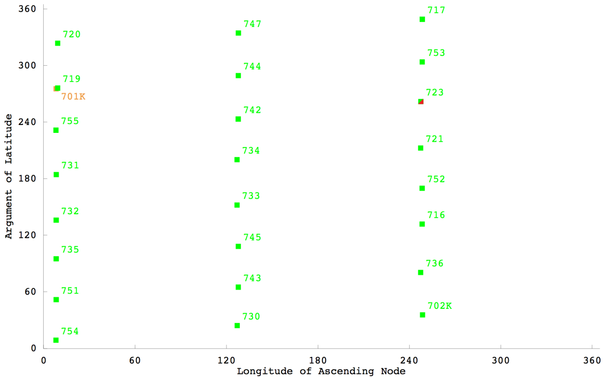
GLONASS Satellite Constellation (GPS Week 1975(951); GPS Seconds 0)
