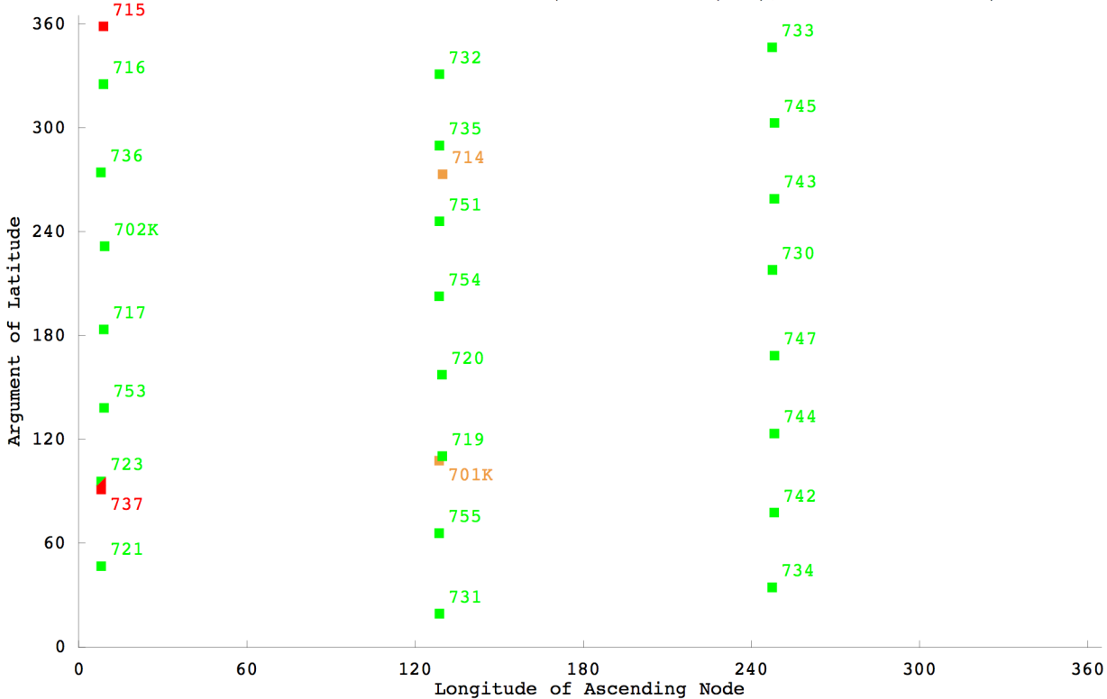
GLONASS Satellite Constellation (GPS Week 1958(934); GPS Seconds 86400)
