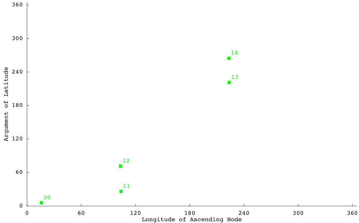
Compass MEO Satellite Constellation (GPS Week 1707(683); GPS Seconds 518415)
