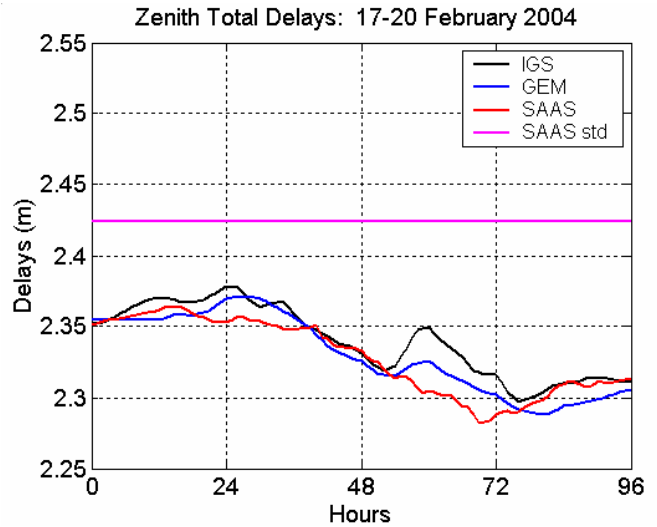
Figure 6: zenith delay profiles
