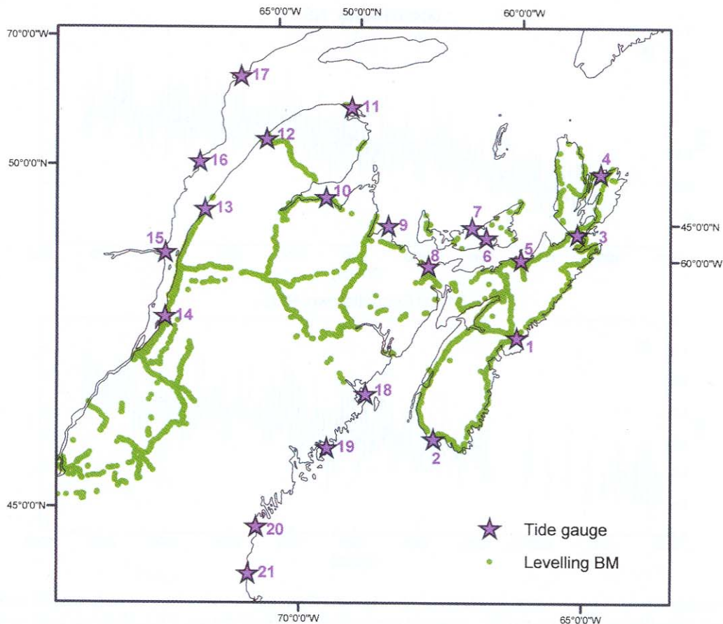
Fig. 1. (Color) Data distribution used in computations. Stars indicate location of tide gauges from which data are employed in analysis of secular sea level change. Releveled segments are shown by their leveling BMs.
