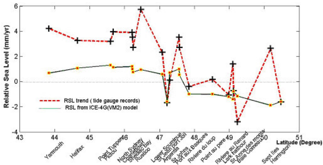
Figure 2: Present day rates of relative sea level change based on tide gauge records (short dashed line) and theoretically predicted rates using the ICE-4G deglaciation history and VM2 structure (solid line).
