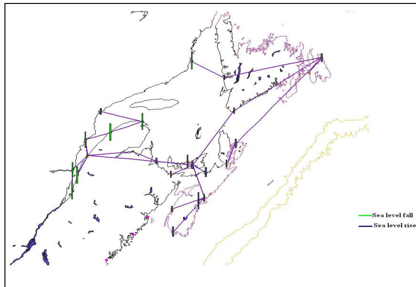
Figure 1: Topology of tide gauge differencing in eastern Canada, along with the profile of sea level changes.
