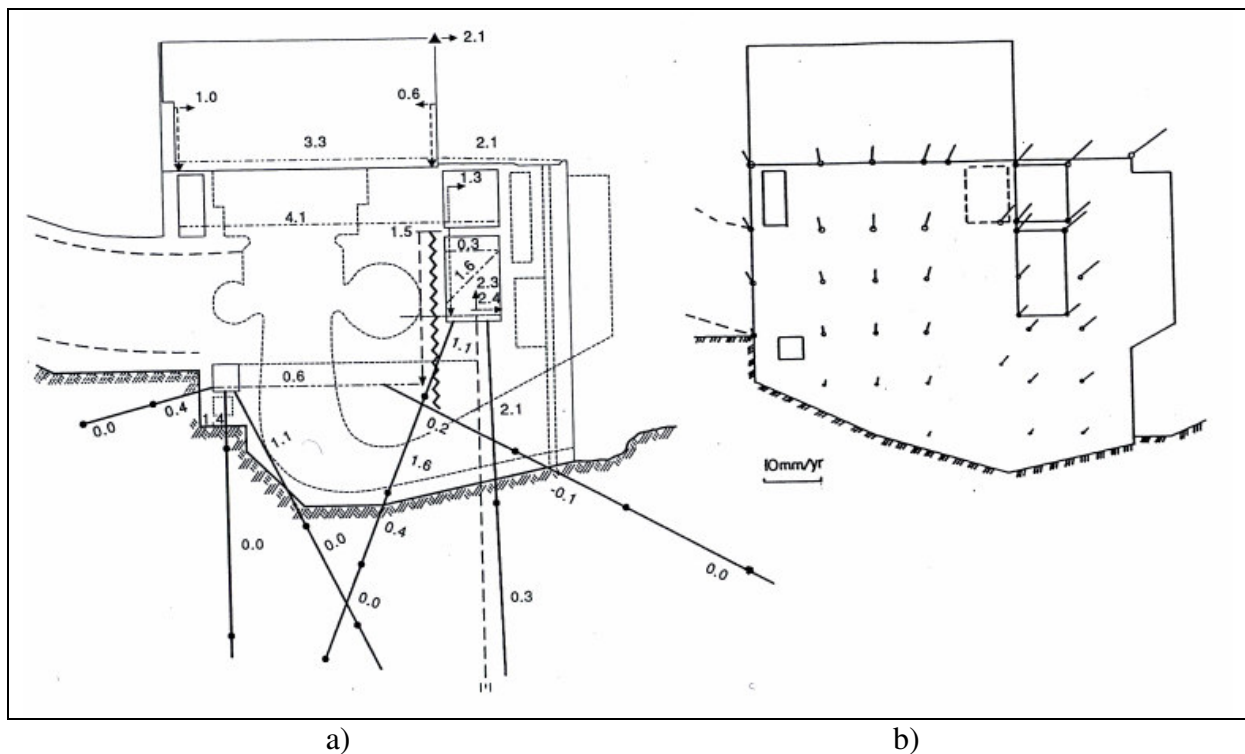
Figure 1: Application of the Generalized Method of geometrical analysis (after Chrzanowski, 1993): a) observed rates of deformation (mm/y), b) derived displacement field.
