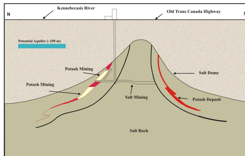
Fig. 5: Geological cross-section
