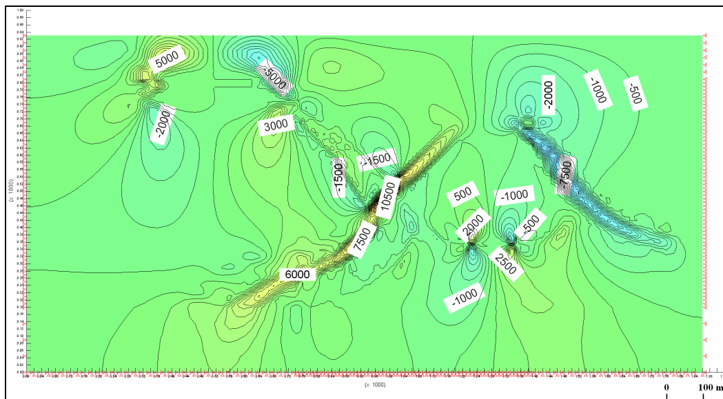
Fig. 7: Distribution of maximum shearing stress (MPa)
