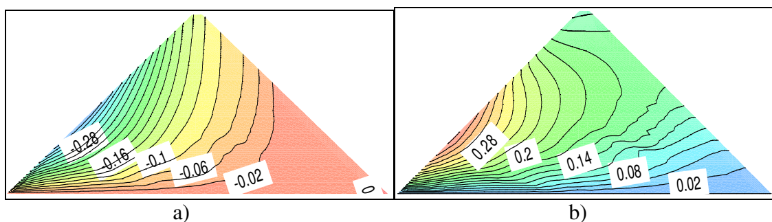
Figure 2: Predicted displacements [m] after filling the reservoir a) vertical displacements b) horizontal displacements
