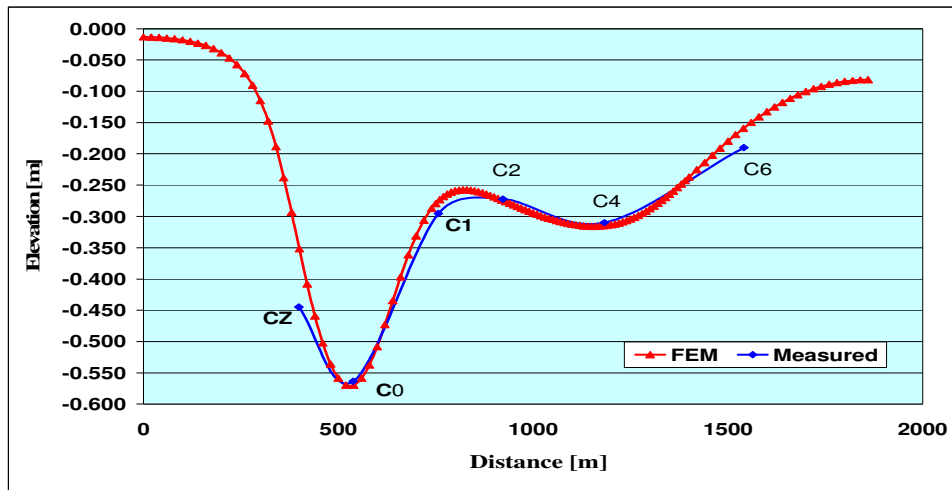
Fig.6: Measured and FEM Surface Subsidence
