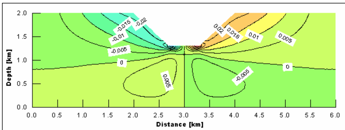
Fig. 4: Horizontal displacement [m].
