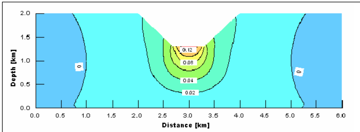
Fig.3: Vertical displacement (m)
